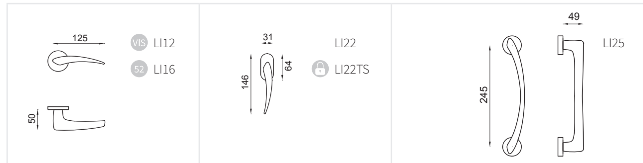
PCS Power cromosat Power satin chrome
