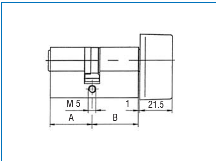
Knob cylinder 8804
